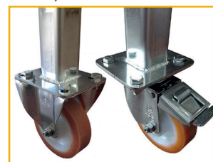
4 wheels, 2 of which with brakes
