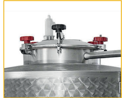
Upper manhole with Vent Valve
