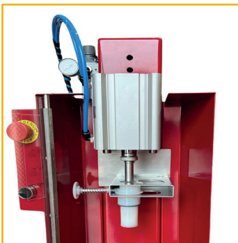
Cone for inserting a cork cap
