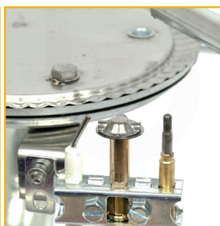
Piezoelectric Unit, Safety, Pilot Flame
